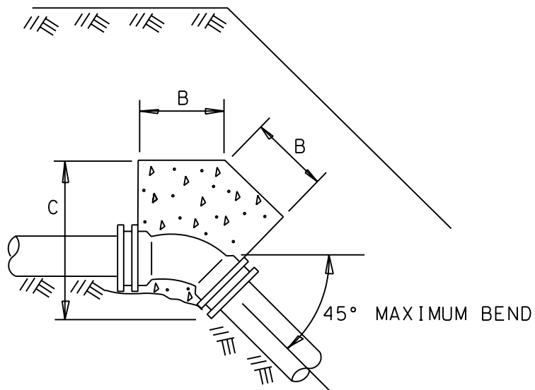
ELEVATION TYPICAL VERTICAL BEND
