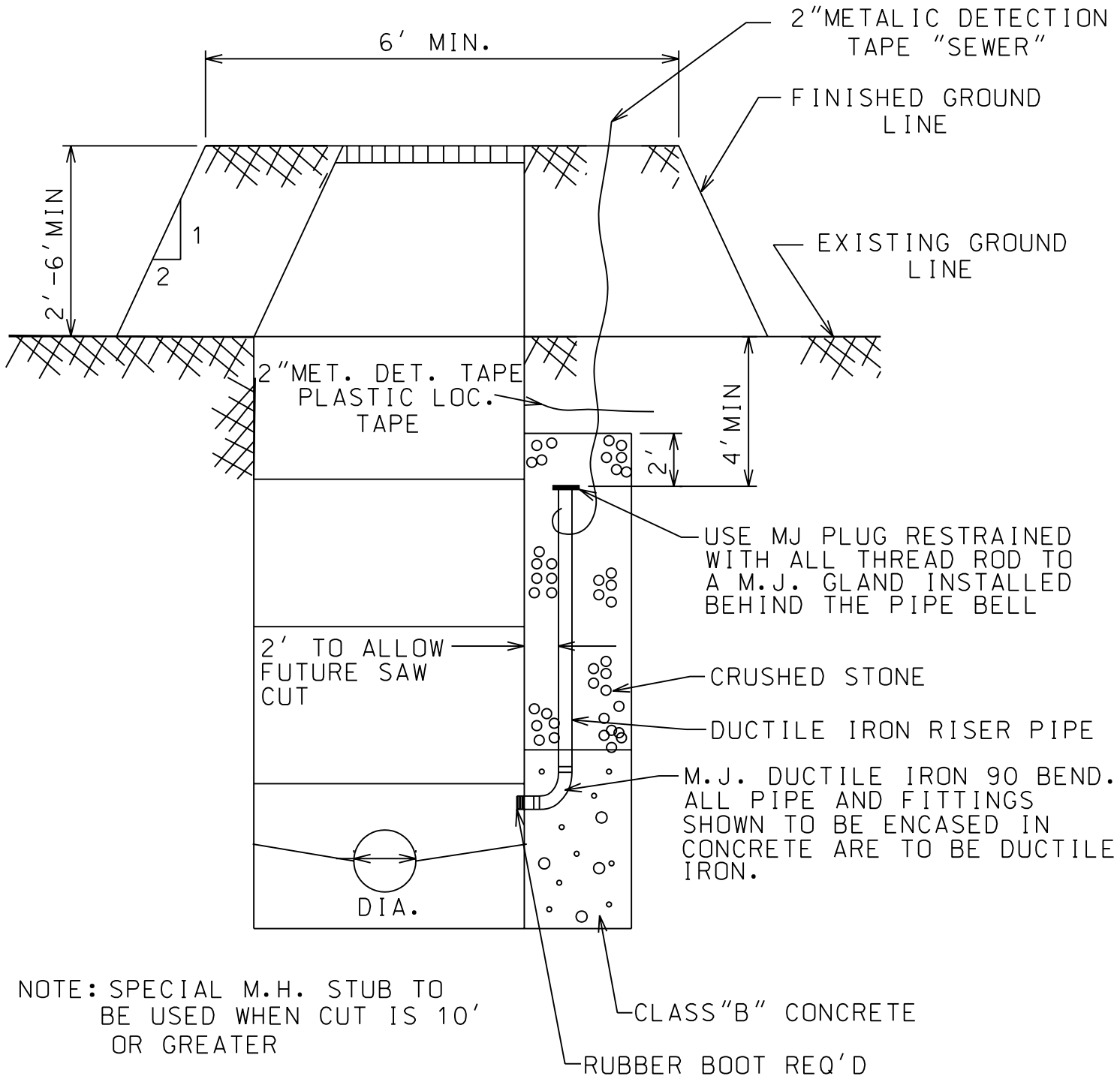
SPECIAL M.H. STUB DETAIL N.T.S.
